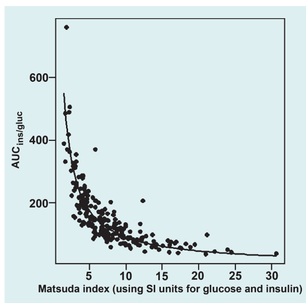
FIGURE 1 Plot of hyperbolic relationship between the ratio of the area-under-the-insulin-curve to the area-under-the-glucose-curve (AUC ins/gluc ) (insulin secretion) and Matsuda index (insulin sensitivity), the component measures of the insulin secretion–sensitivity index-2 (ISSI-2).
